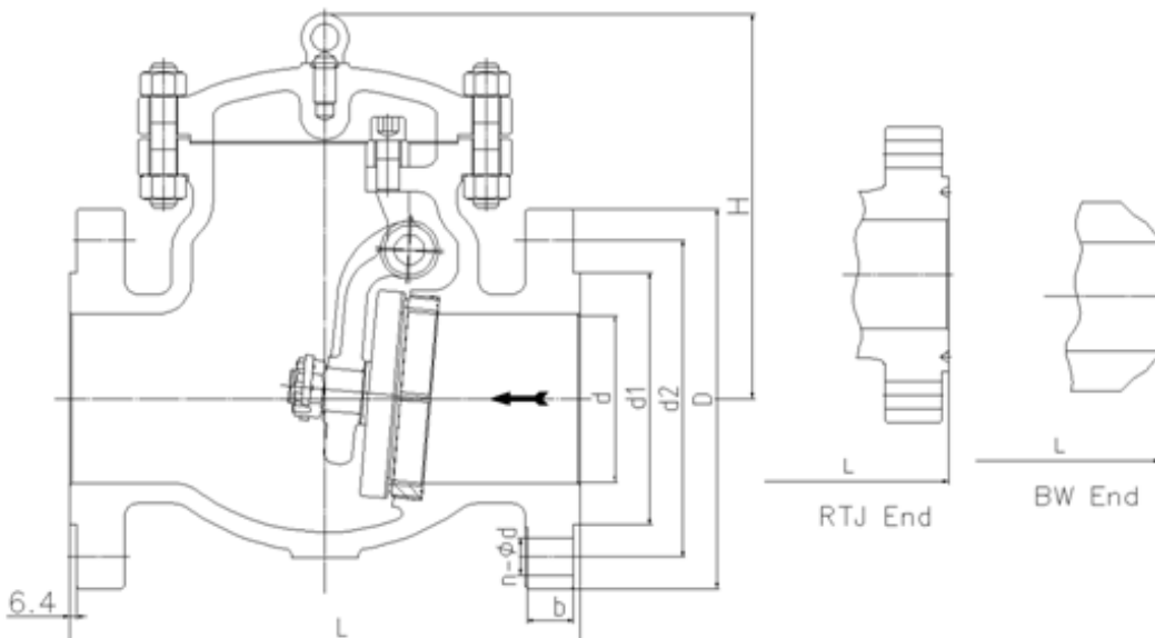
Class900 Alloy Check Valves
