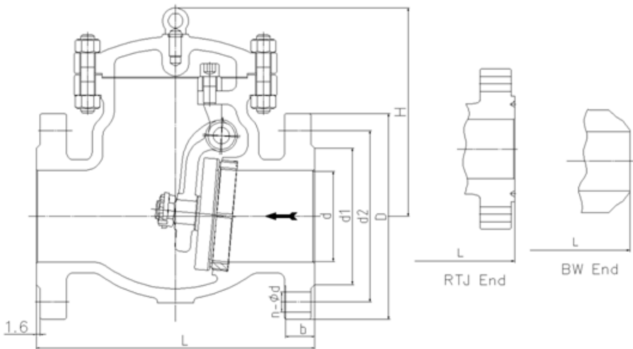
Class300 Cryogenic checkvalve
