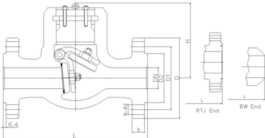
Class1500 Cryogenic check valve
