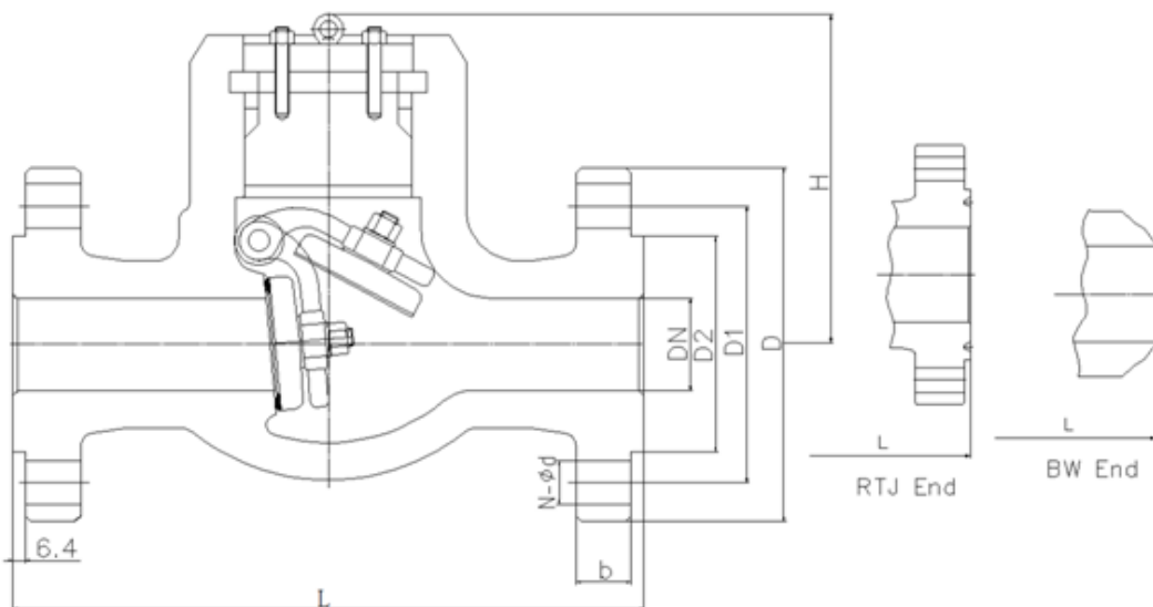
Class2500 Cryogenic check valve
