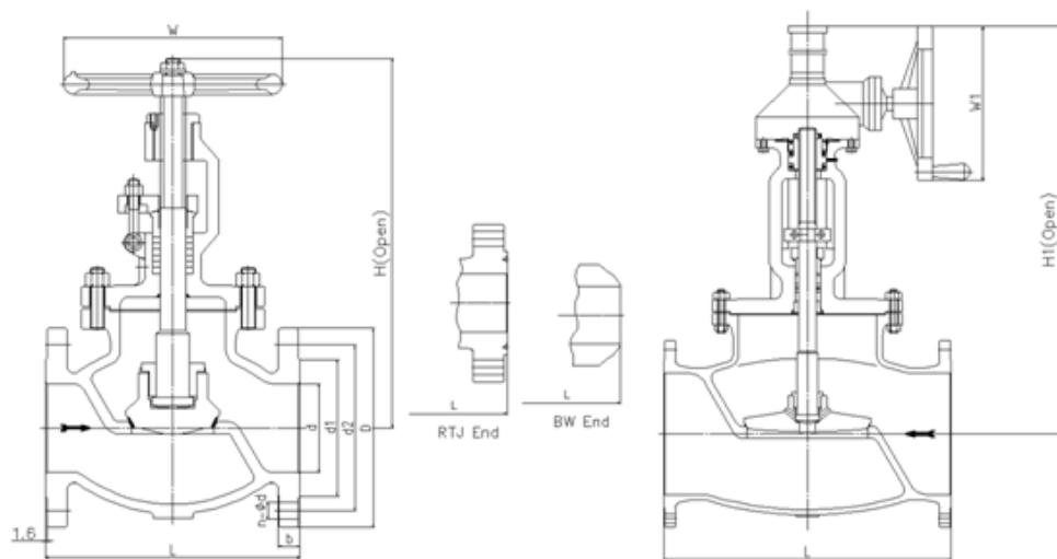
Class300 Low Emission Globe valve
