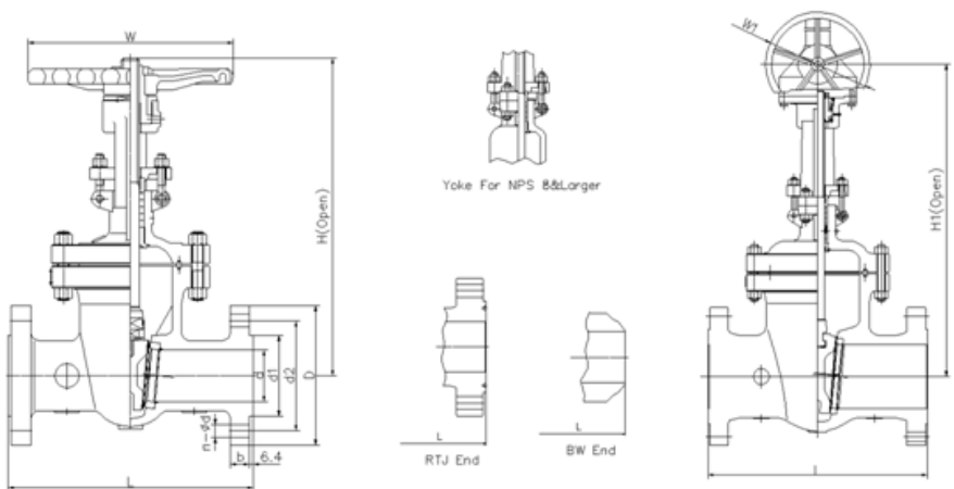
Class900 Wedge Gate Valve
